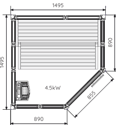
IMPRESSION SAUNA I1515/c Size : W1495 × D1495 × H2090 mm
