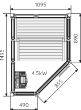
IMPRESSION SAUNA I1115/c Size : W1095 × D1495 × H2090 mm
