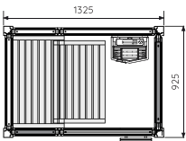
IMPRESSION SAUNA I1309 Size : W1325 × D925 × H2090 mm
